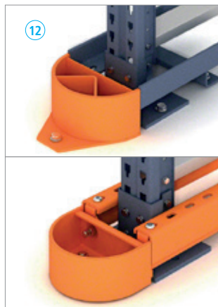
Guide rail and protector
